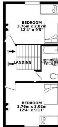
1ST FLOOR 31.63 sq. m. ( 340.46 sq. ft. )
