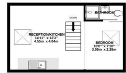
2ND FLOOR 100 SQ. FT. (9.3 SQ. M.) APPROX.
